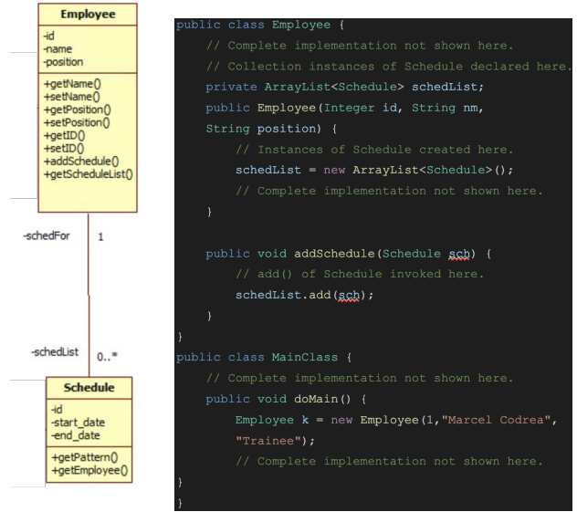
(a) Extract from the model of project 4. (b) Visualization of corresponding code part from project 4.
